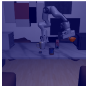
CLIP-only
